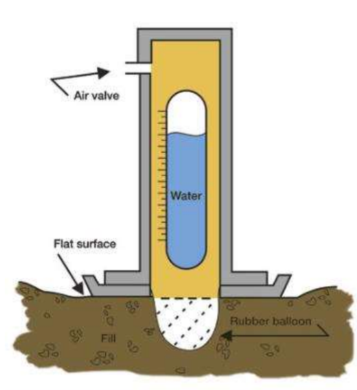
Illustration of the balloon densometer test
