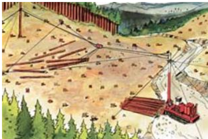
Slack skyline carriage
